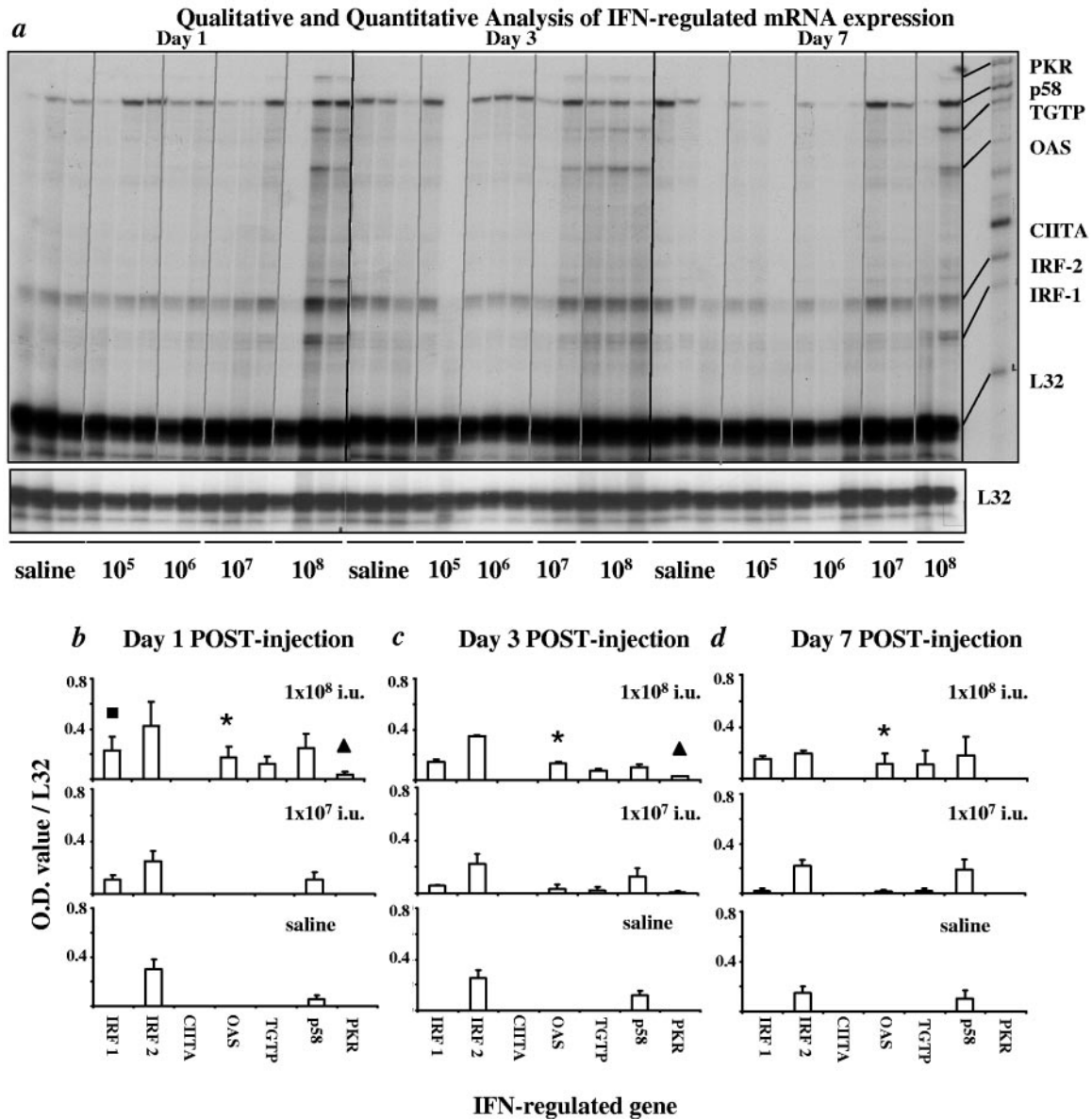
FIG. 1. Analysis of IFN-regulated mRNA expression. (a) RPA gel showing bands corresponding to mRNAs of IFN-regulated mRNAs 1 day (left panel), 3 days (middle panel), and 7 days (right panel) after intracranial injection of RAD35. Dosages of RAD35 ( 1 \times 10^5 to 1 \times 10^8 ) or saline are shown below the lanes. Sizes of individual IFN-regulated mRNA probes are indicated at the far right. (b to d) Quantification of IFN-regulated mRNA expression using ImageJ software. The band intensity was determined by dividing the optical density (OD) value for each IFN-regulated mRNA by the OD value for the L32 control in each lane and was expressed as a percentage. To obtain a representative reading of the denser L32 bands, these bands were exposed overnight (lower L32 image), while for readings from the other mRNAs, the gels were exposed for 5 days. (b) Quantification of IFN-regulated mRNA expression 1 day after CNS injection of saline or 1 \times 10^7 to 1 \times 10^8 IU of RAD35. (c) Quantification of IFN-regulated mRNA expression 3 days after CNS injection of saline or 1 \times 10^7 to 1 \times 10^8 IU of RAD35. (d) Quantification of IFN-regulated mRNA expression 7 days after CNS injection of saline or 1 \times 10^7 to 1 \times 10^8 IU of RAD35. *, P < 0.1 compared to control (saline) OAS value; ▲, P < 0.1 compared to control PKR value; ■, P < 0.1 compared to control IRF-1 value at each time point. Quantification of expression after the injection of 1 \times 10^5 to 1 \times 10^6 IU of virus is not illustrated because changes were not statistically significant. We only show expression below ( 1 \times 10^7 IU) and above ( 1 \times 10^8 IU) the threshold of induction of statistically significant increases in mRNA expression.
